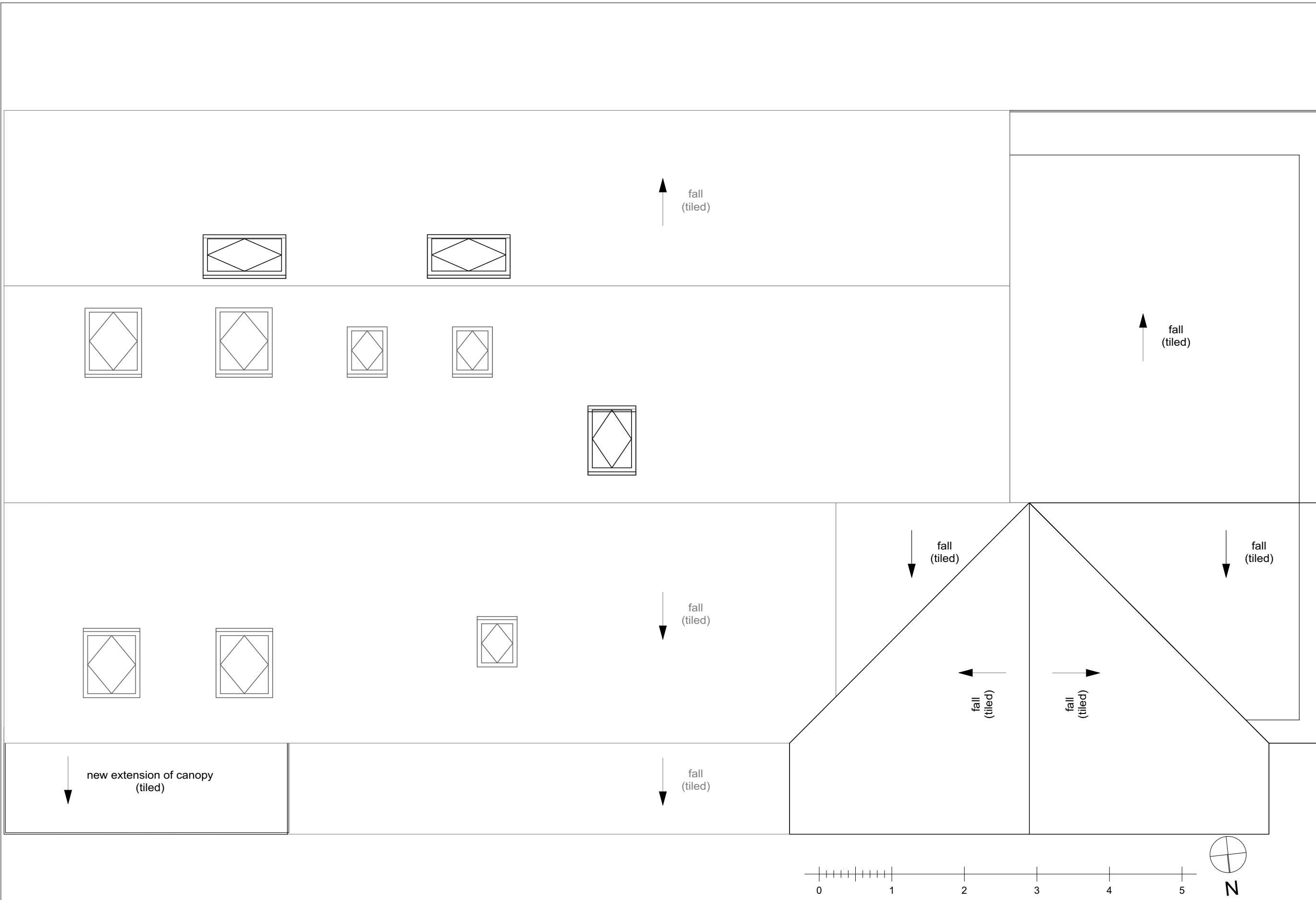
Roof Plan - Proposed 1:50
